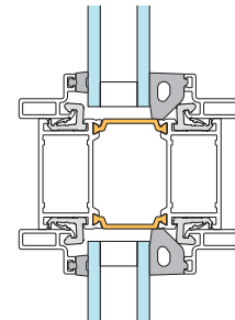
Glastjocklek 20-30 mm
